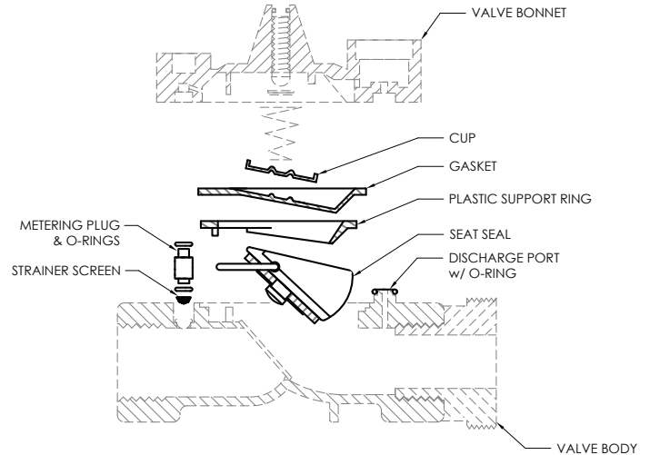
EXPLODED SIDE VIEW
